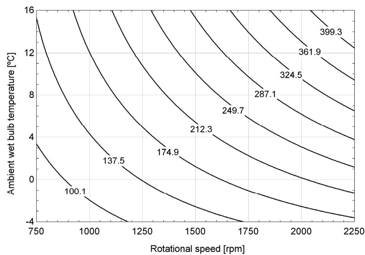
Figure 6. Iso-lines of heating capacity of the ASHPWH.
